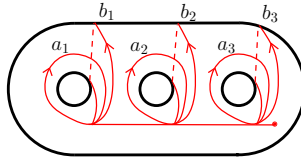
Figure 4. Generators a_j, b_j of \pi_1(\Sigma_3)
