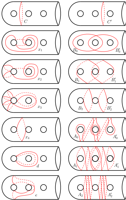
Figure 1. The curves C, x_1, x_2, x_3, x_4, d, e of the first embedding are given on the left. The curves B_0, B_1, B_2, A_0, A_1, A_2 of the second embedding (except for C , which is already given on the left) and C', B'_0, B'_1, B'_2, A'_0, A'_1, A'_2 of the third embedding are on the right.
