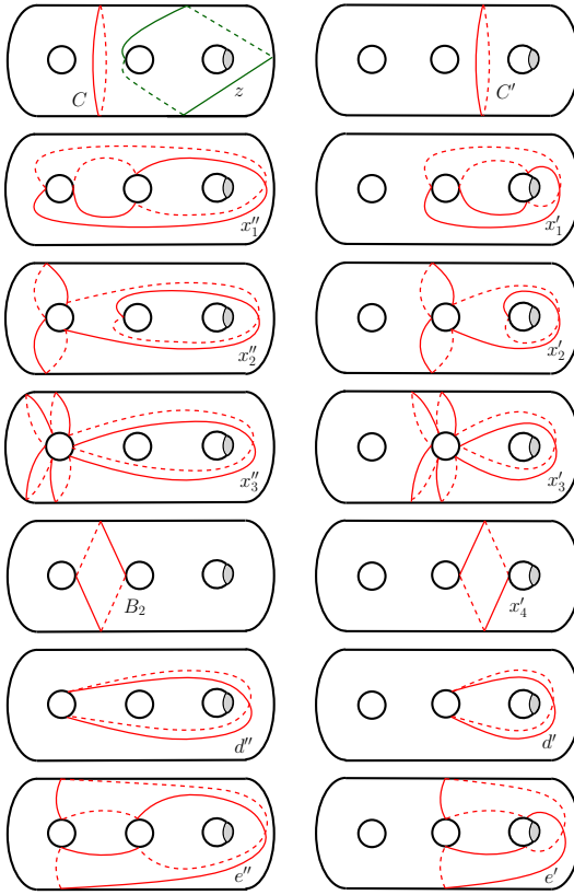
Figure 3. The surface \Sigma_3^1 with shifted boundary. The curves C' , x'_1, x'_2, x'_3, x'_4, d', e' of the second embedding are on the right, and the curves C, x''_1, x''_2, x''_3, B_2, d'', e'' of the third embedding are given on the left. The Dehn twist curve z in the conjugation \phi is on the top left (in green).
